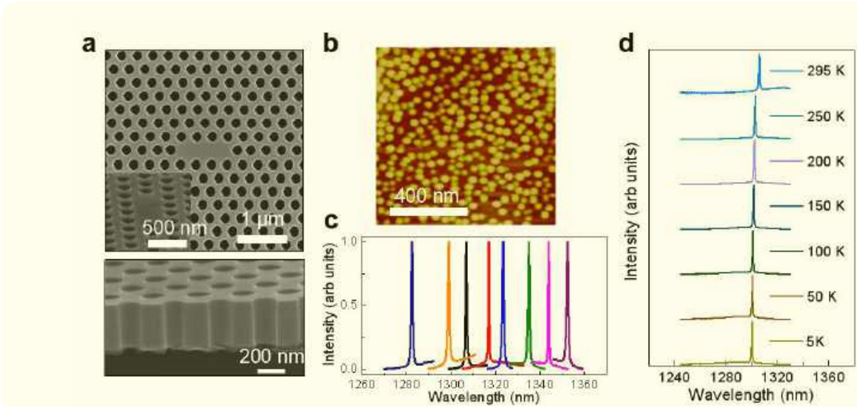
图 2. 硅基量子点激光器器件表征图 Figure 2. The device characteristics.
